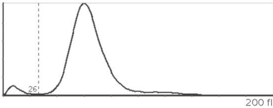
EOS Histogram
